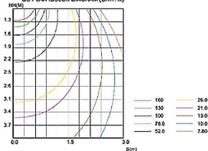
GO PLAN ISOLUX DIAGRAM (UNIT: lx)
